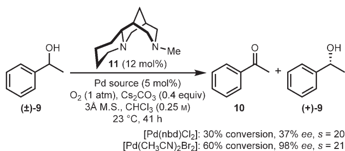
Scheme 2. Kinetic resolution of (±)- 9 with PdX 2 and diamine 11 .
